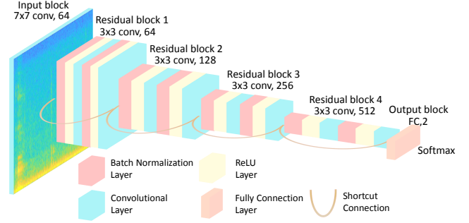
Figure 5: The architecture of the ParkinsonNet. It contains four residual blocks, and each of which contains two convolutional layers.
