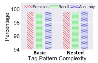
Figure 18: Performance under different tag complexities.
